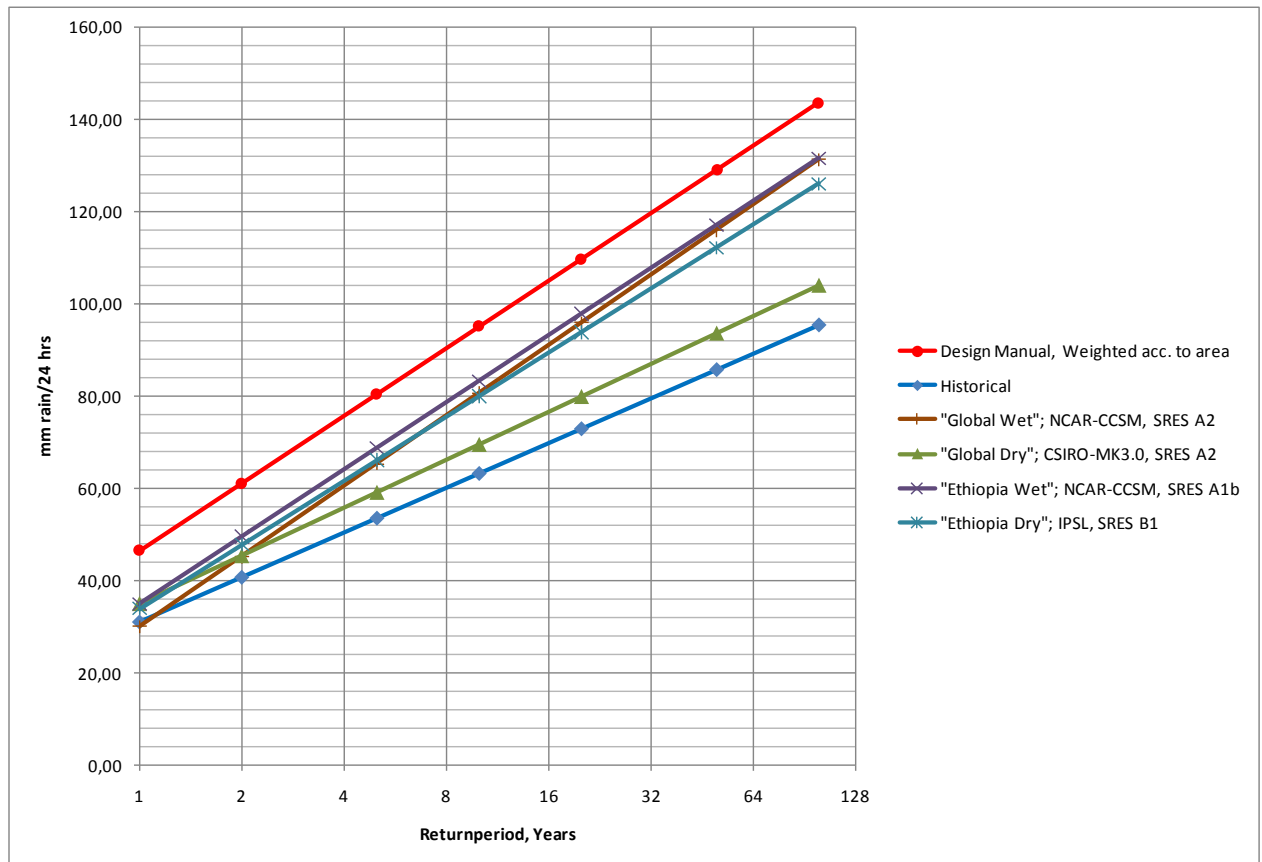
Figure 2-15 Calculated design curves
