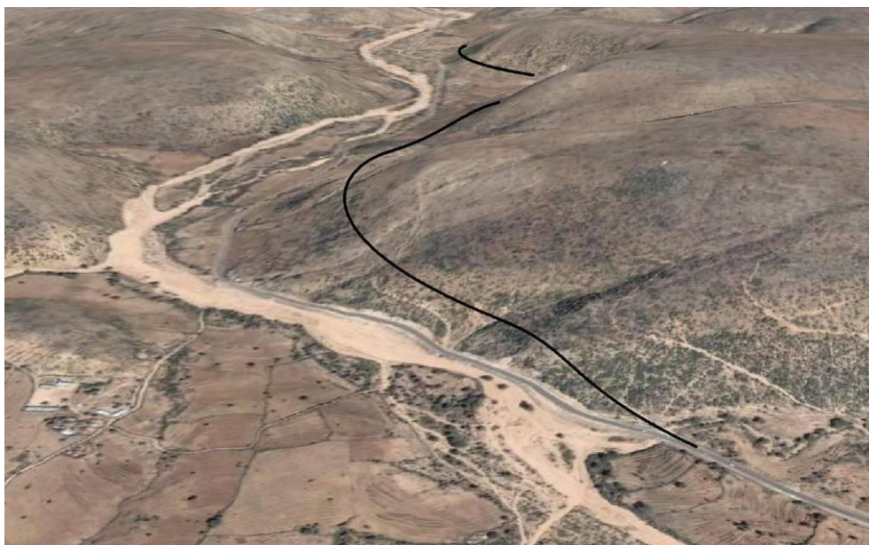
Figure 4-22 Alternative roadway alignment out of flood limits Dire Dawa Region
