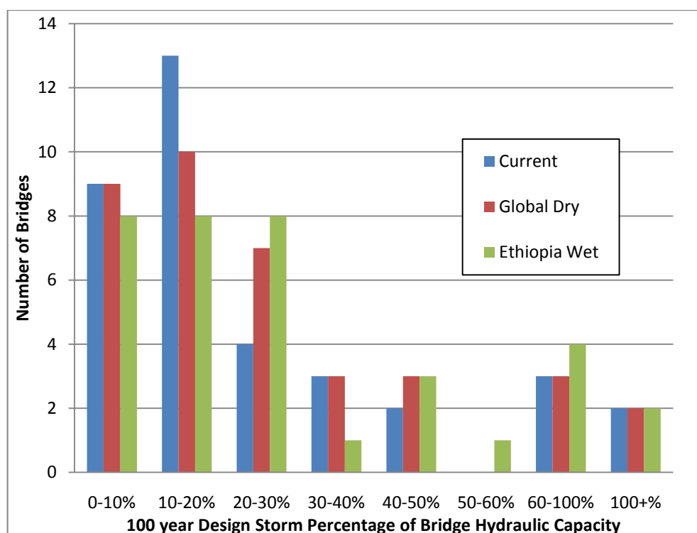
Figure 4-1 Mekele Abi Adi Adwa Bridge Hydraulic Capacities under 100 year storm
