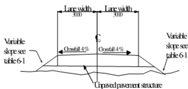
Normal section of design standard DS6
