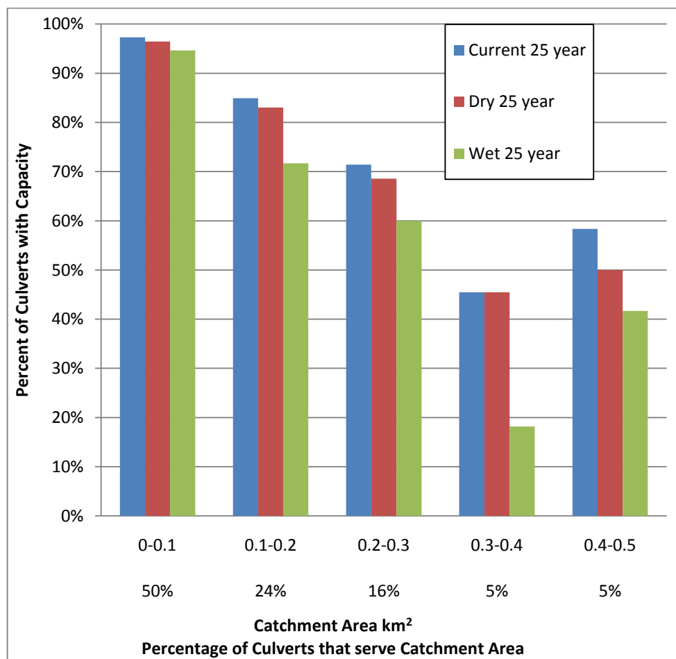
Figure 4-8 Percent of culverts with capacity for a 25 year storm with a Hw:D<1.5 compared to catchment area
