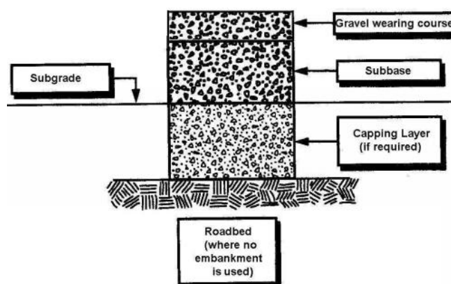
Figure 3-7 Typical elements of a gravel road DS6
