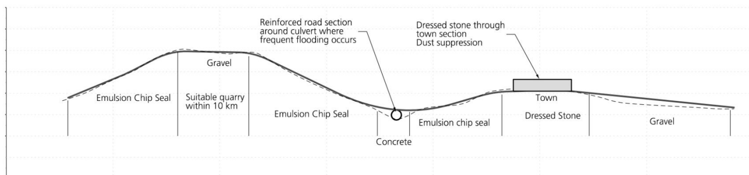
Figure 4-14 Climate resilient gravel road
