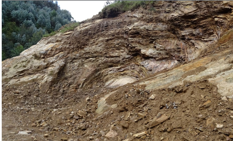
Figure 6: Highly folded, foliated and weathered gneissic road-side outcrop.
