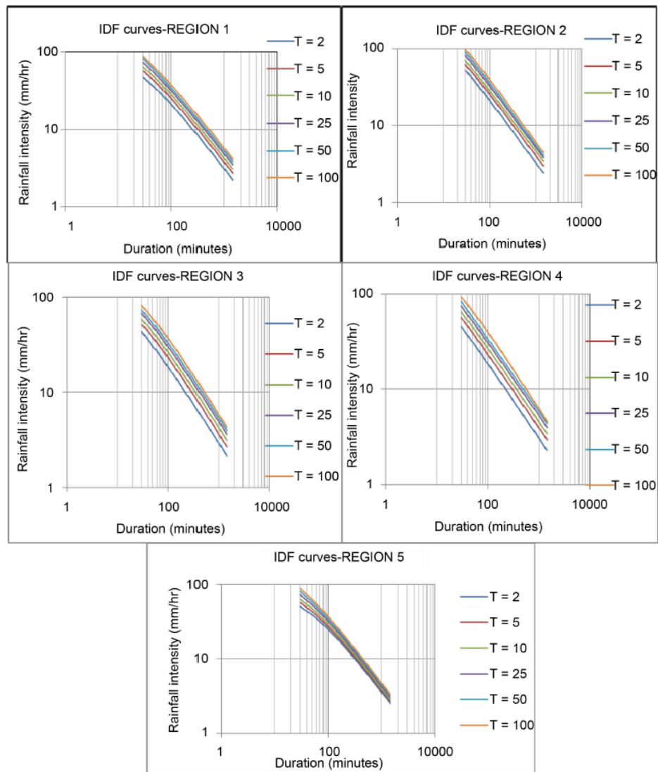
Figure 33: Regional IDF curves for selected return period.
